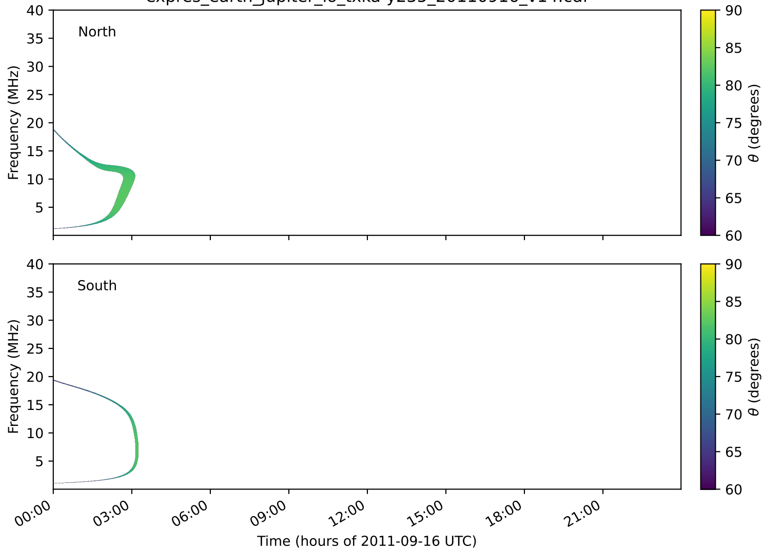
expres_earth_jupiter_io_txka-y235_20110916_v14.cdf
