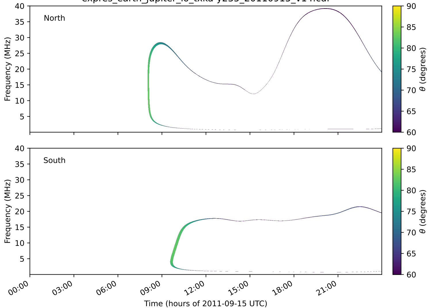
expres_earth_jupiter_io_txka-y235_20110915_v14.cdf
