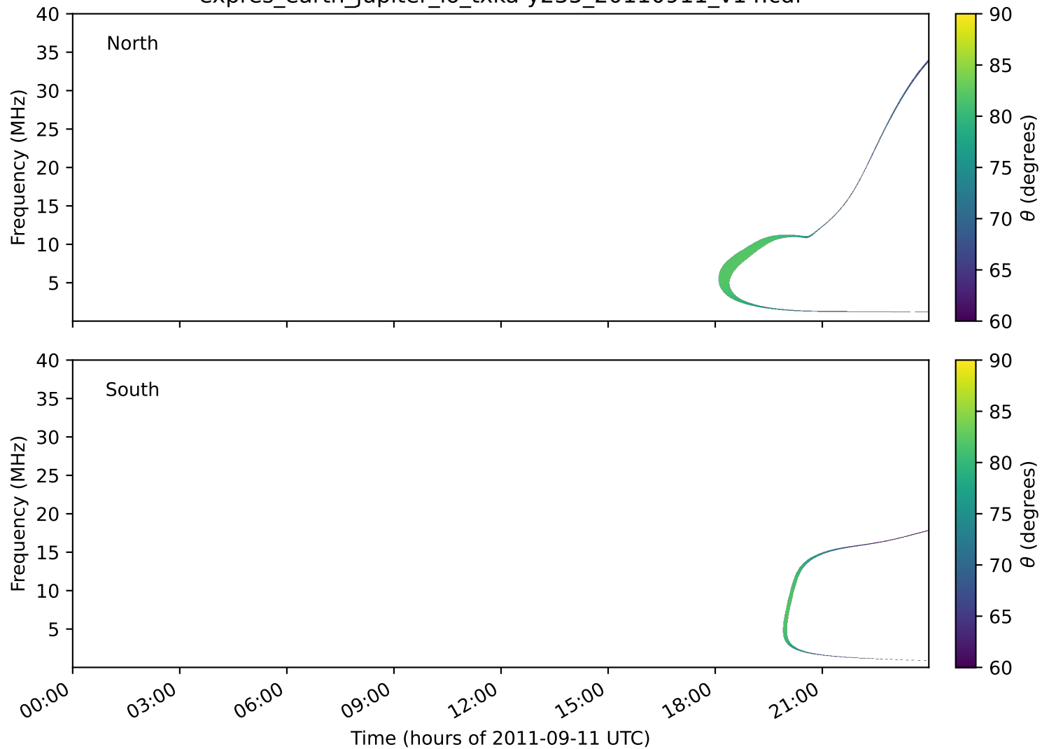
expres_earth_jupiter_io_txka-y235_20110911_v14.cdf
