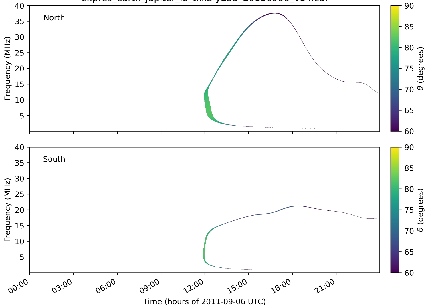
expres_earth_jupiter_io_txka-y235_20110906_v14.cdf
