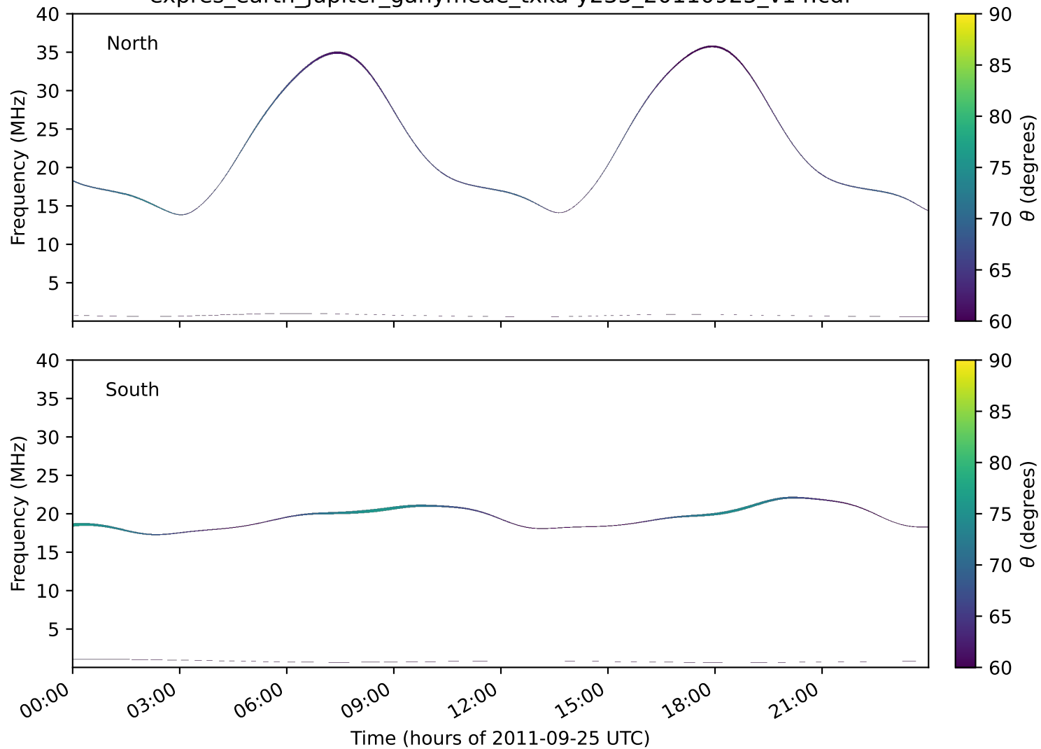
expres_earth_jupiter_ganymede_txka-y235_20110925_v14.cdf
