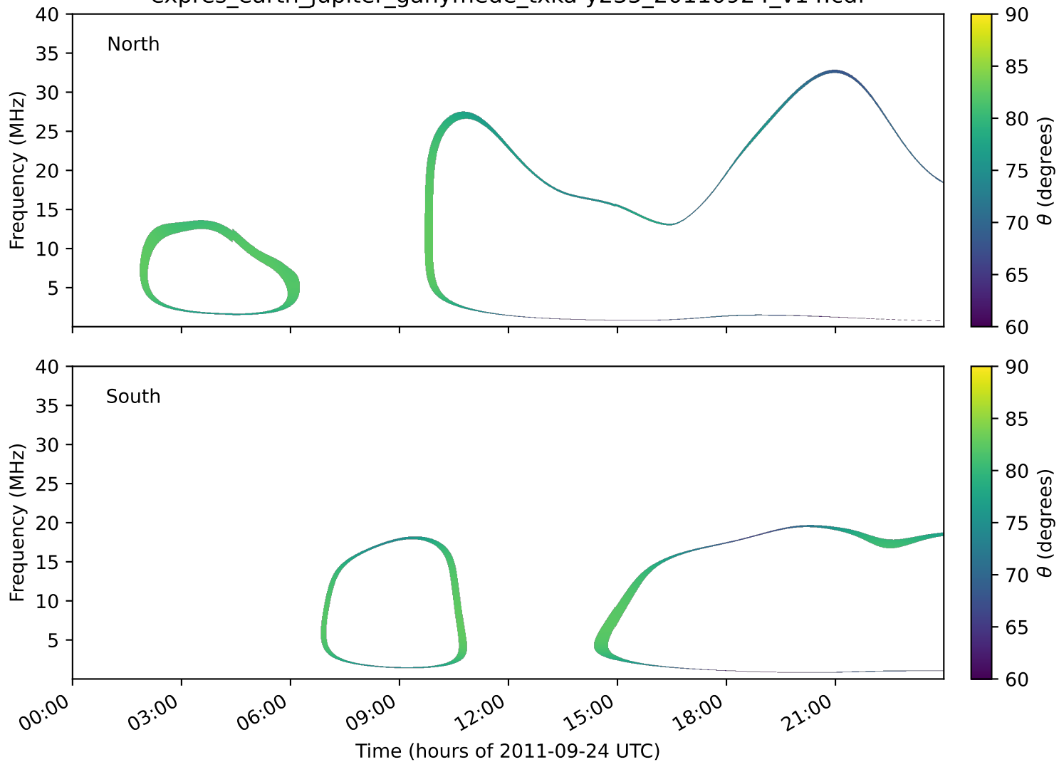
expres_earth_jupiter_ganymede_txka-y235_20110924_v14.cdf
