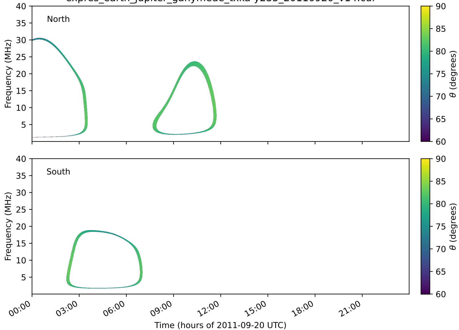
expres_earth_jupiter_ganymede_txka-y235_20110920_v14.cdf
