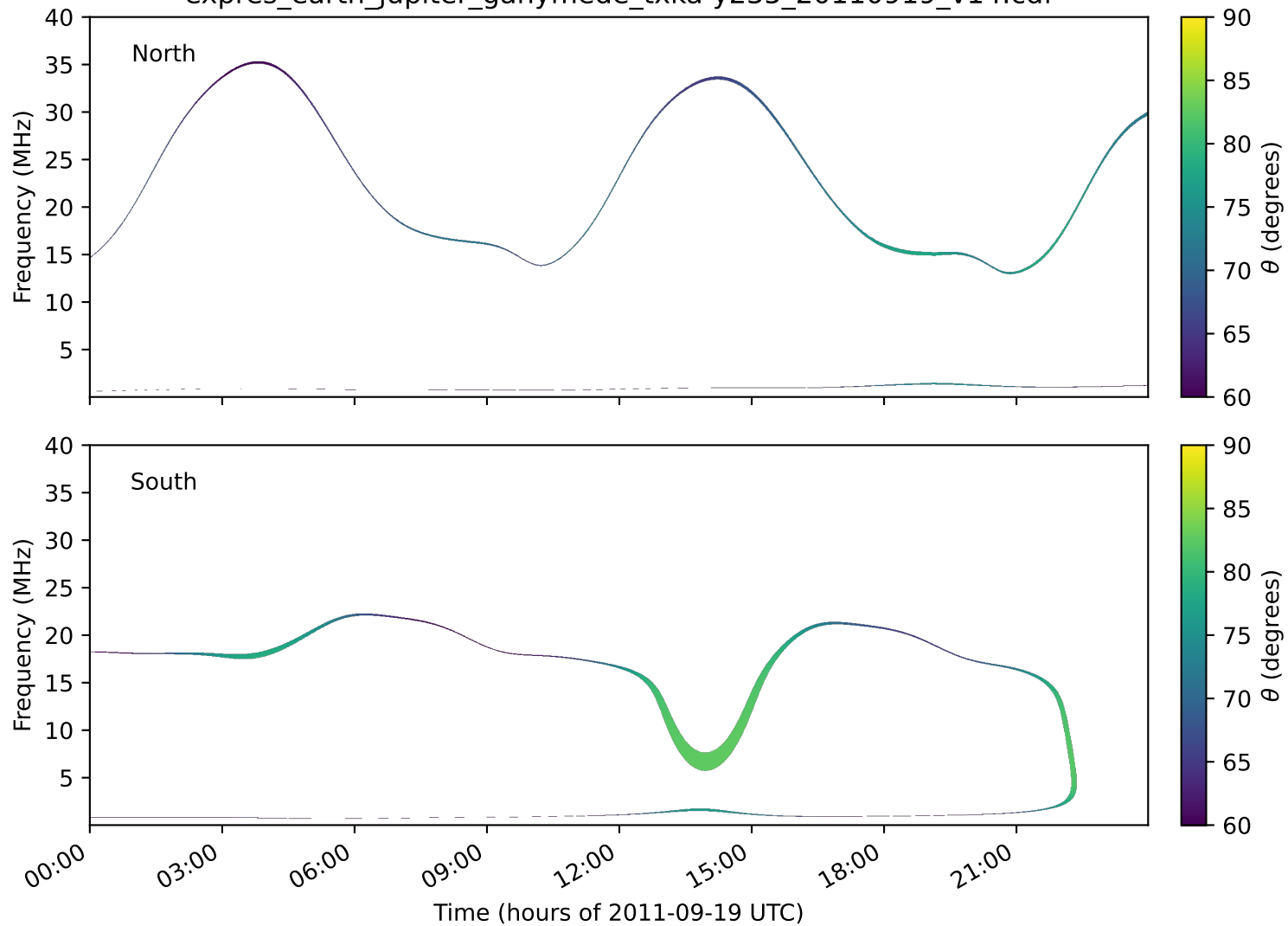
expres_earth_jupiter_ganymede_txka-y235_20110919_v14.cdf
