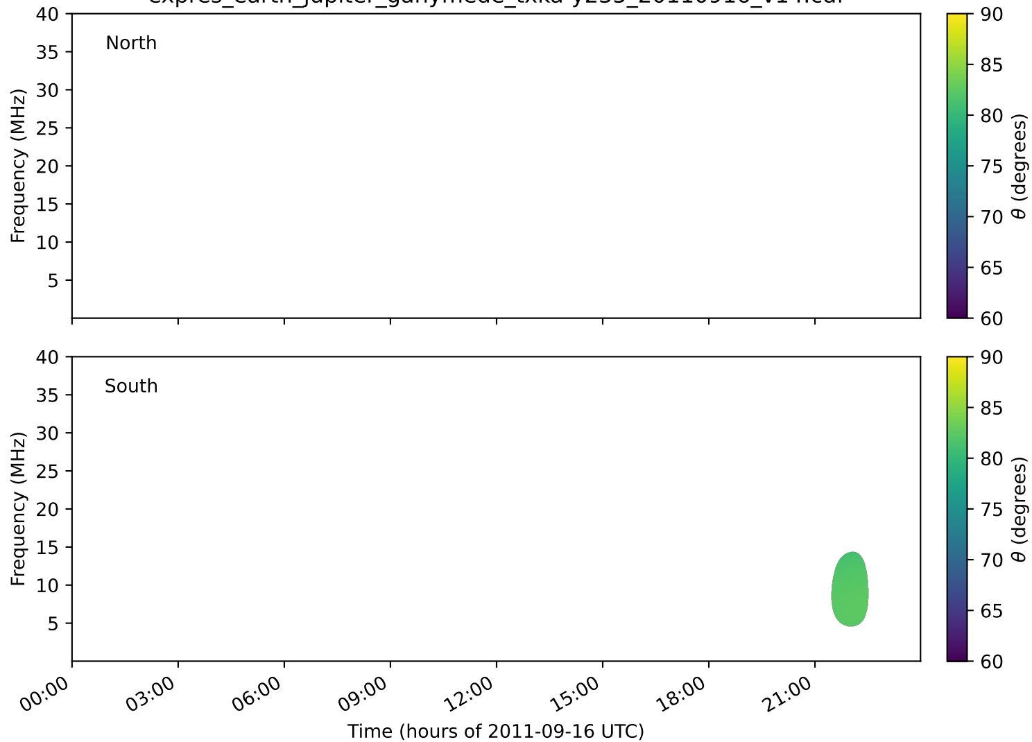
expres_earth_jupiter_ganymede_txka-y235_20110916_v14.cdf
