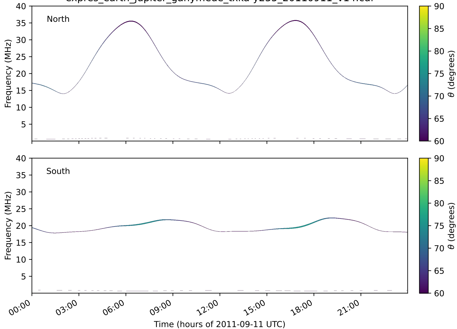
expres_earth_jupiter_ganymede_txka-y235_20110911_v14.cdf
