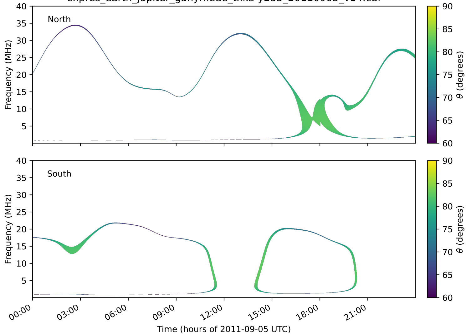
expres_earth_jupiter_ganymede_txka-y235_20110905_v14.cdf
