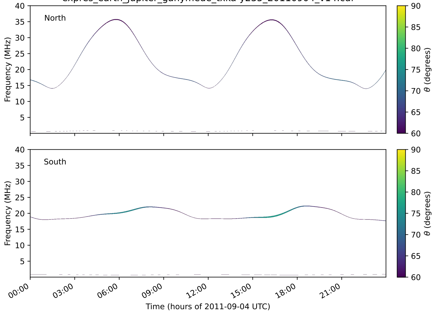
expres_earth_jupiter_ganymede_txka-y235_20110904_v14.cdf
