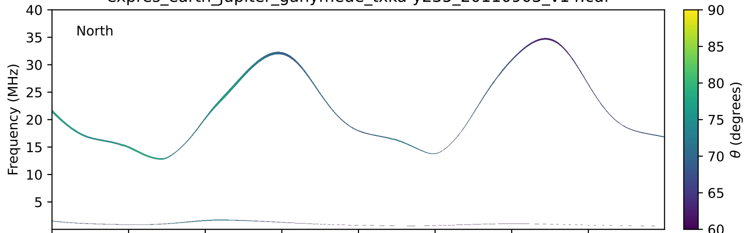
expres_earth_jupiter_ganymede_txka-y235_20110903_v14.cdf
