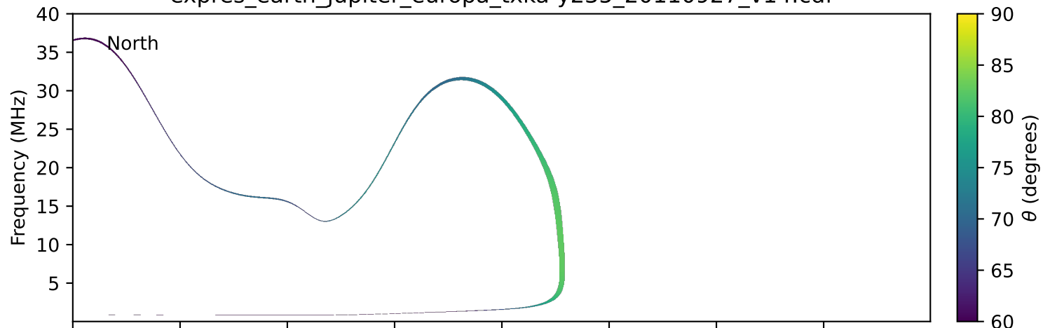
expres_earth_jupiter_europa_txka-y235_20110927_v14.cdf
