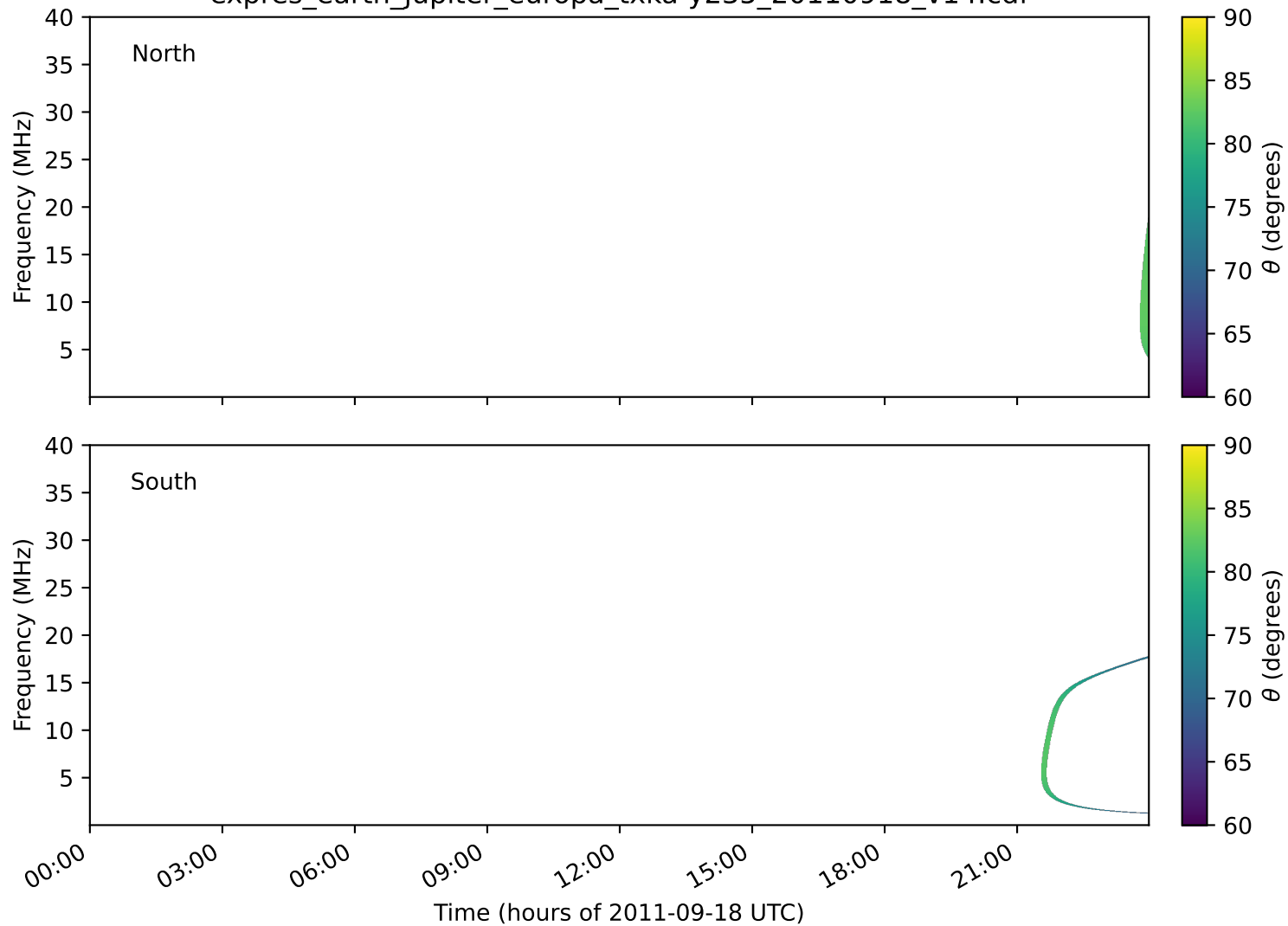
expres_earth_jupiter_europa_txka-y235_20110918_v14.cdf
