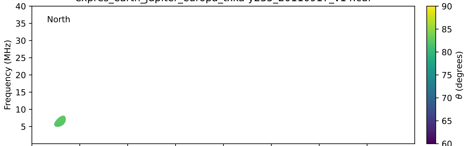
expres_earth_jupiter_europa_txka-y235_20110917_v14.cdf
