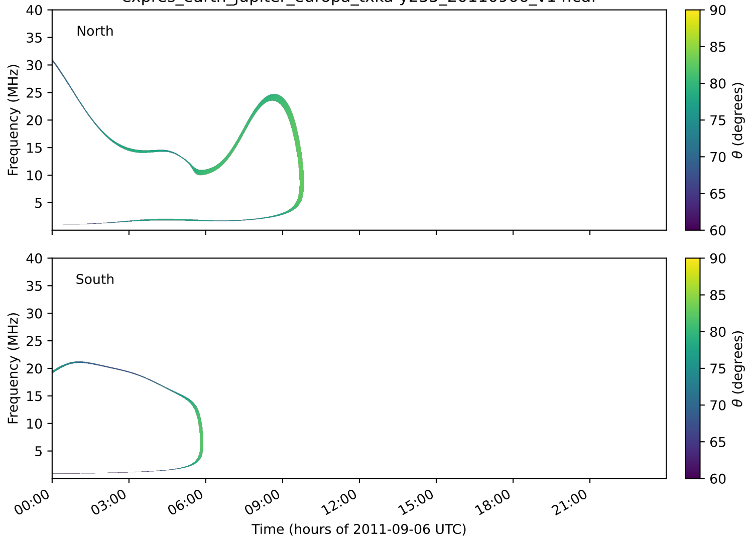
expres_earth_jupiter_europa_txka-y235_20110906_v14.cdf
