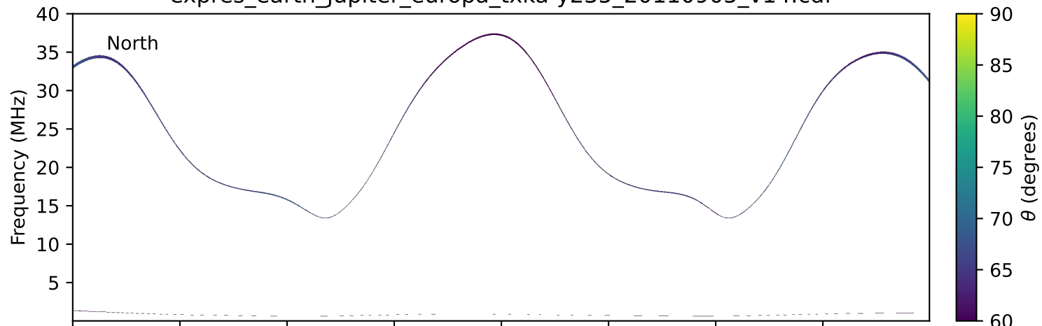
expres_earth_jupiter_europa_txka-y235_20110905_v14.cdf
