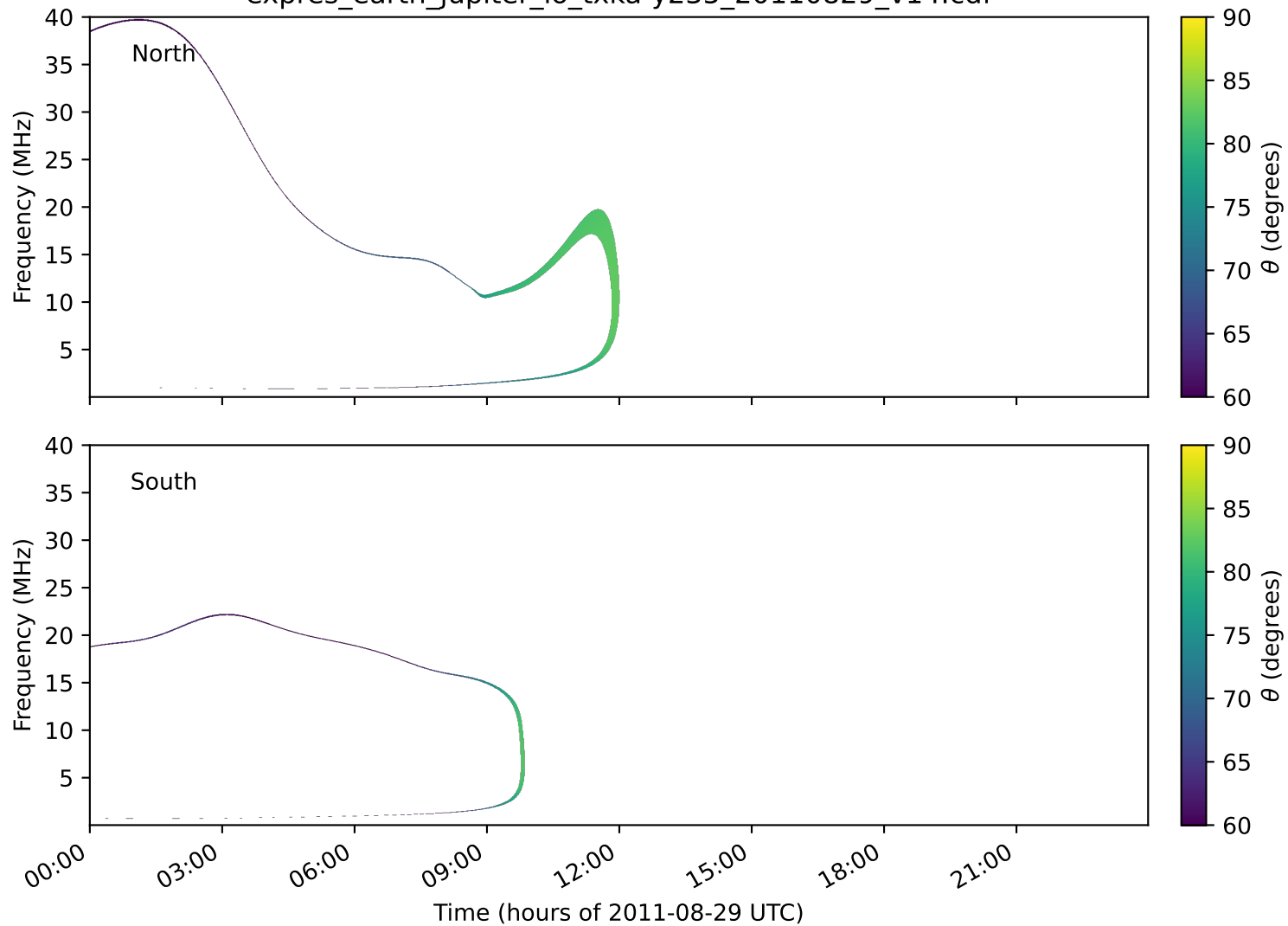
expres_earth_jupiter_io_txka-y235_20110829_v14.cdf
