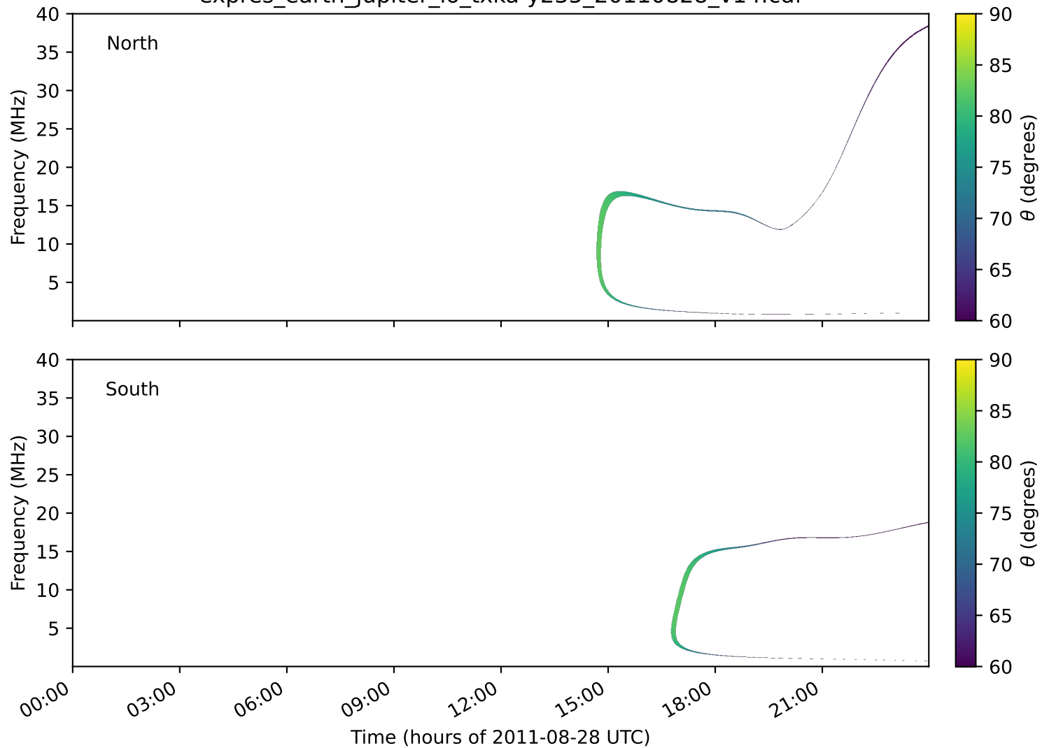
expres_earth_jupiter_io_txka-y235_20110828_v14.cdf
