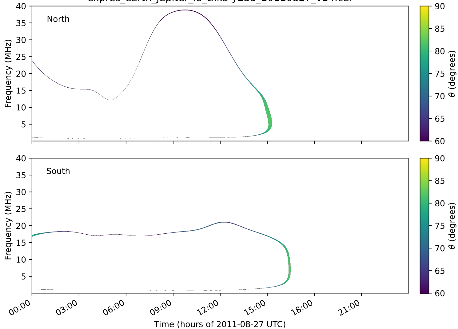
expres_earth_jupiter_io_txka-y235_20110827_v14.cdf
