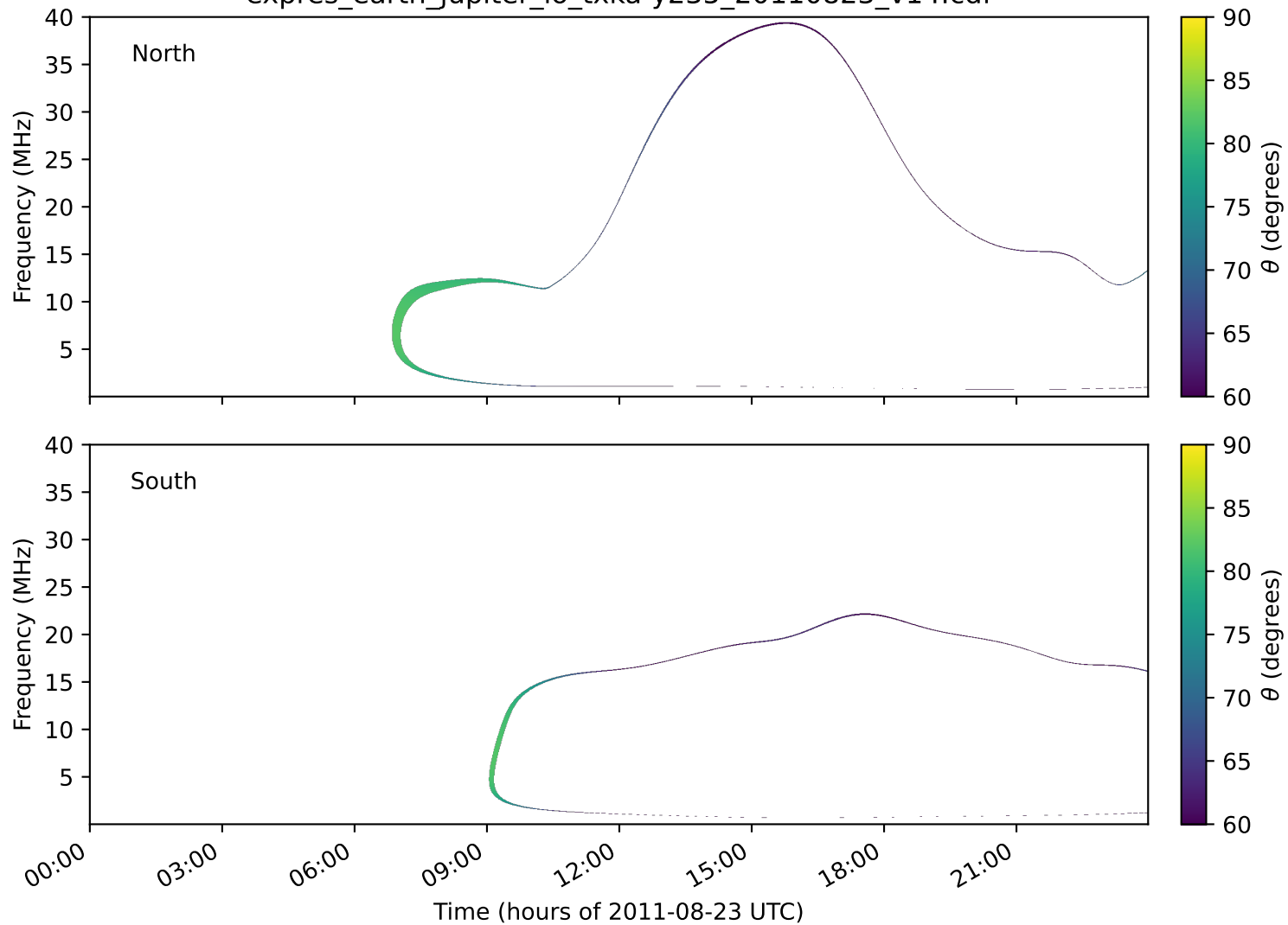
expres_earth_jupiter_io_txka-y235_20110823_v14.cdf
