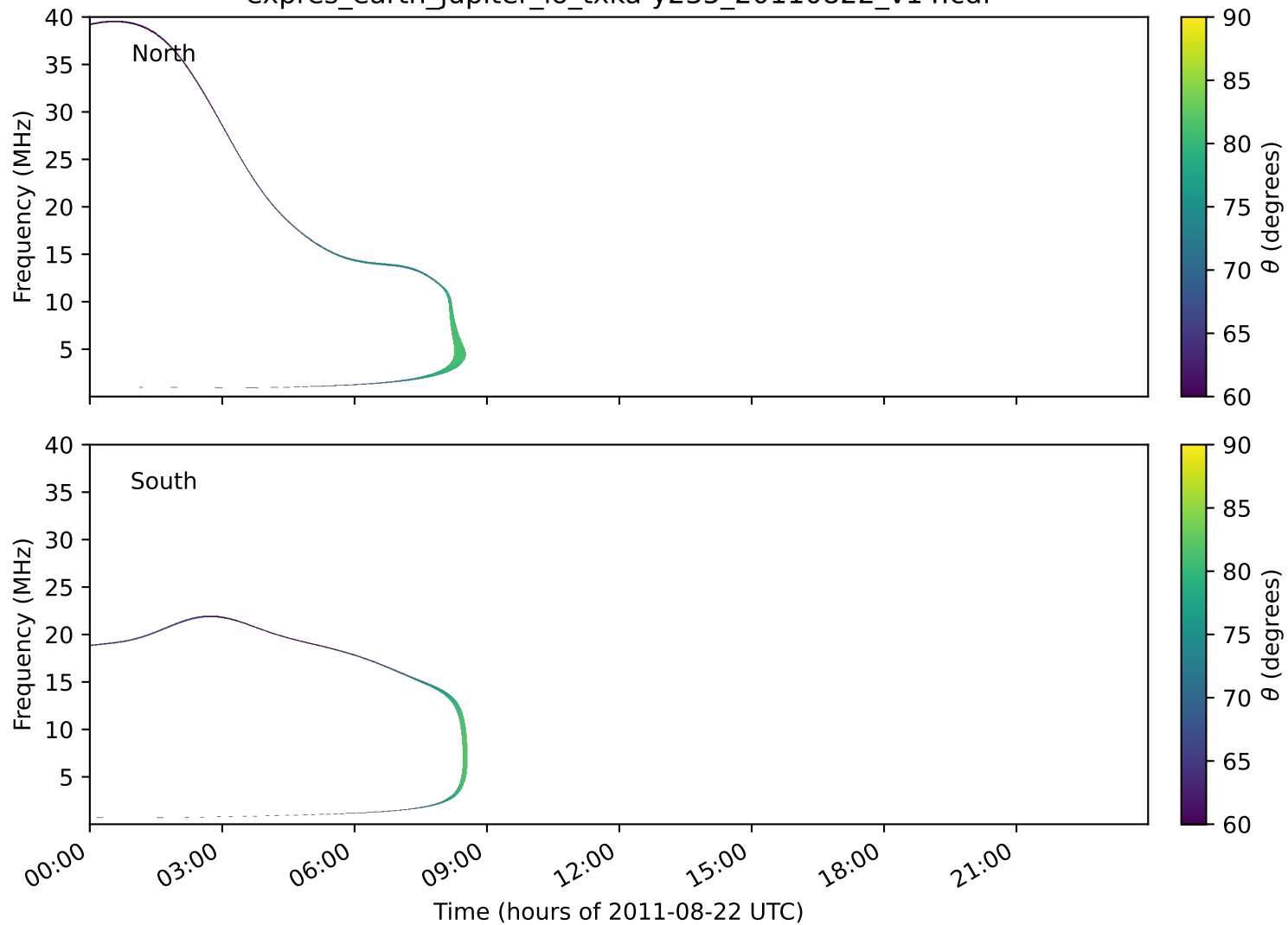
expres_earth_jupiter_io_txka-y235_20110822_v14.cdf
