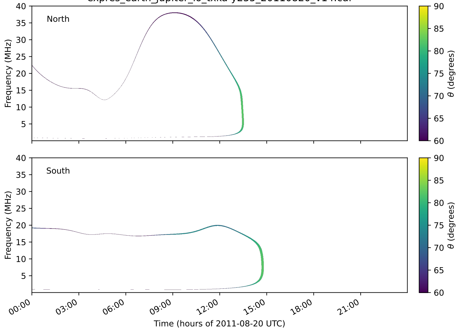
expres_earth_jupiter_io_txka-y235_20110820_v14.cdf
