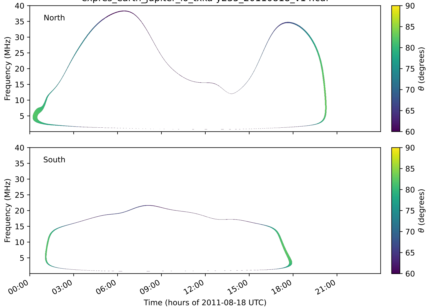
expres_earth_jupiter_io_txka-y235_20110818_v14.cdf
