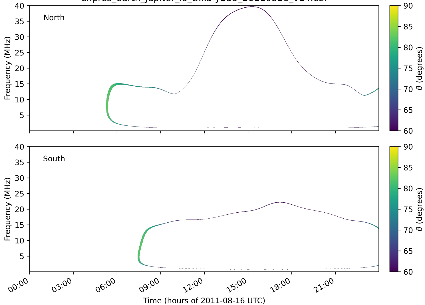
expres_earth_jupiter_io_txka-y235_20110816_v14.cdf
