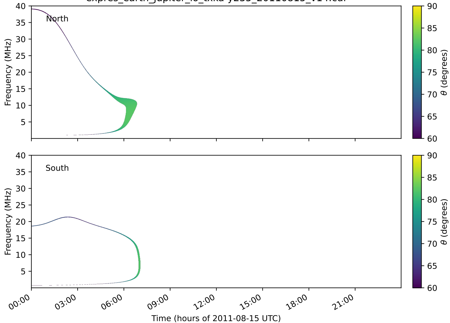
expres_earth_jupiter_io_txka-y235_20110815_v14.cdf
