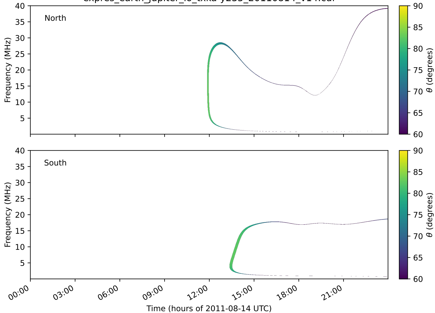
expres_earth_jupiter_io_txka-y235_20110814_v14.cdf
