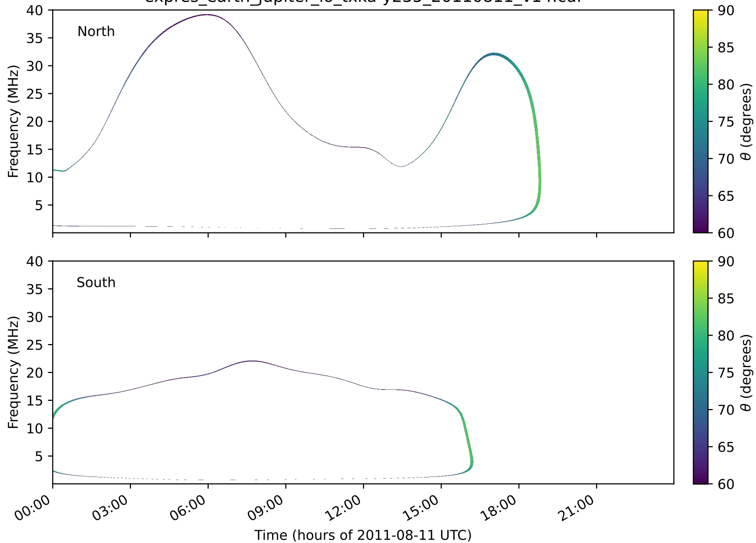
expres_earth_jupiter_io_txka-y235_20110811_v14.cdf
