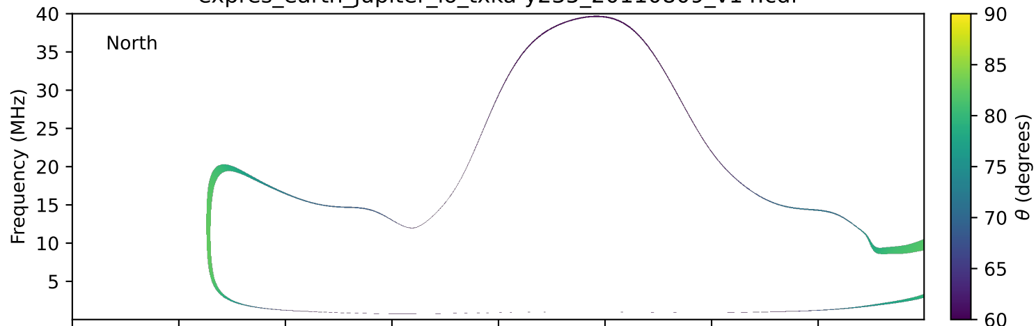
expres_earth_jupiter_io_txka-y235_20110809_v14.cdf
