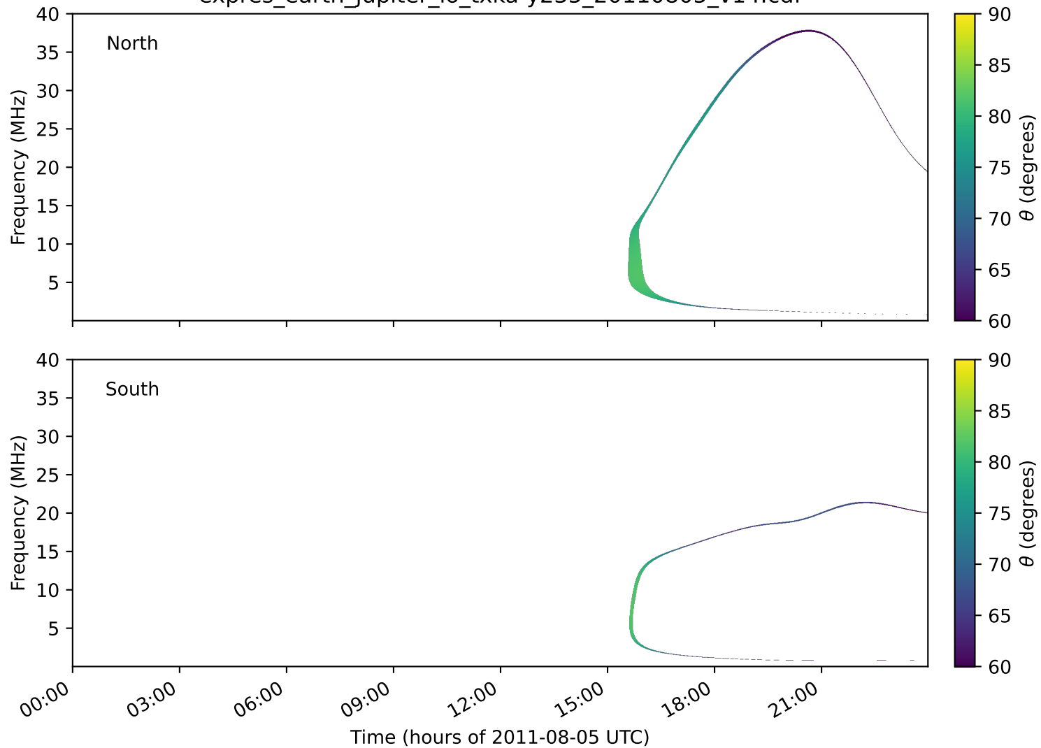
expres_earth_jupiter_io_txka-y235_20110805_v14.cdf
