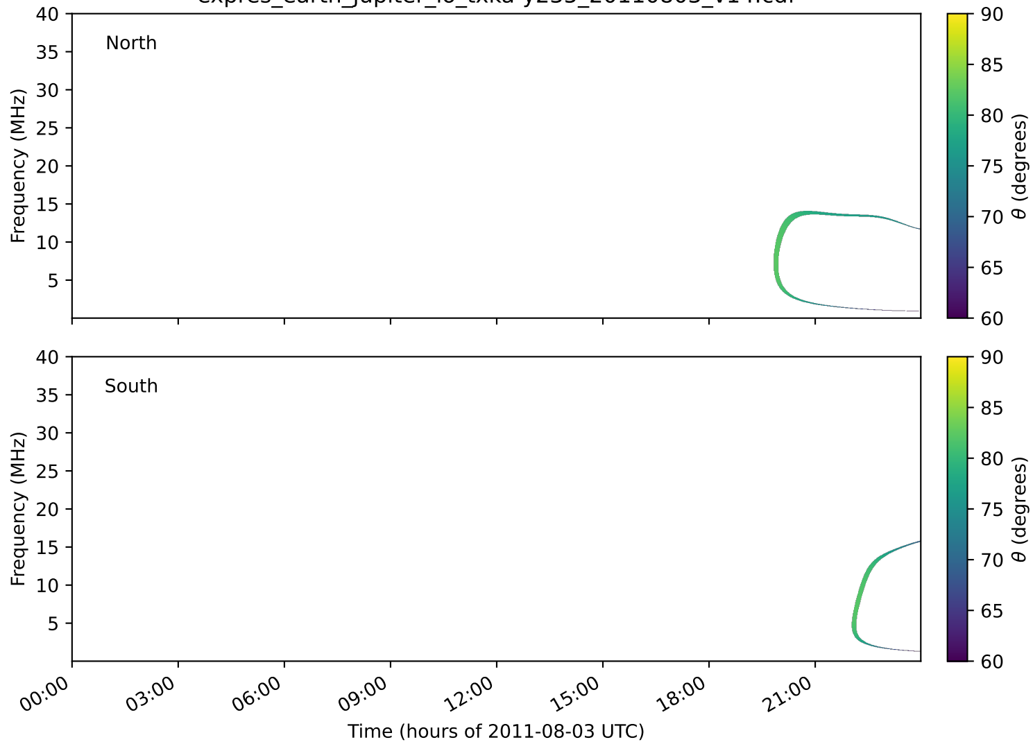
expres_earth_jupiter_io_txka-y235_20110803_v14.cdf
