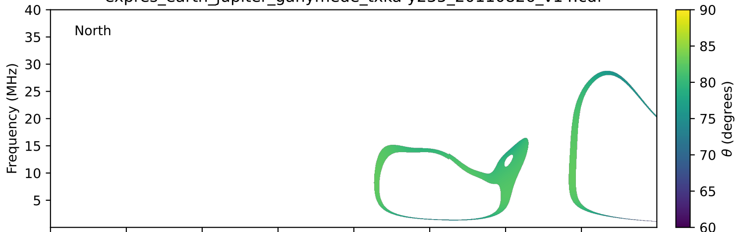
expres_earth_jupiter_ganymede_txka-y235_20110826_v14.cdf
