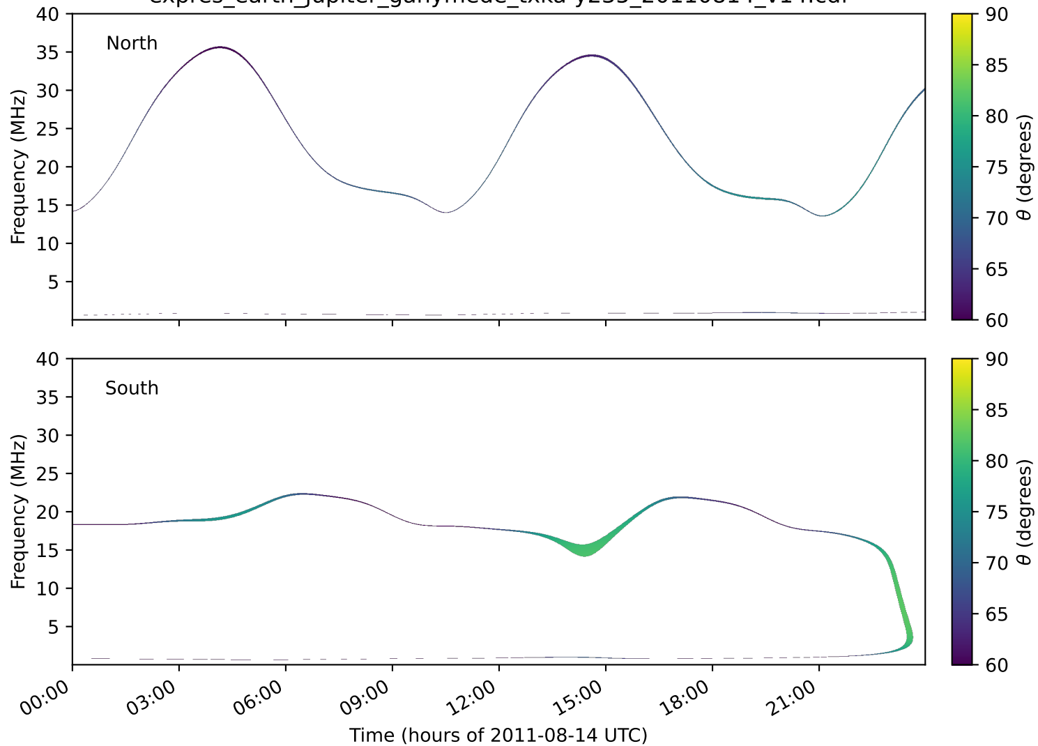
expres_earth_jupiter_ganymede_txka-y235_20110814_v14.cdf
