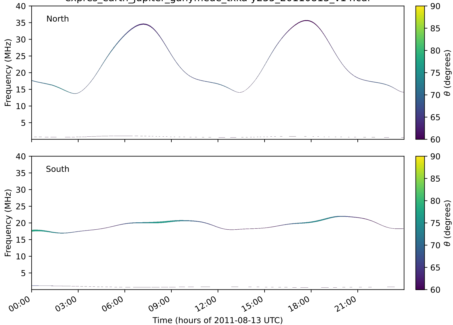
expres_earth_jupiter_ganymede_txka-y235_20110813_v14.cdf
