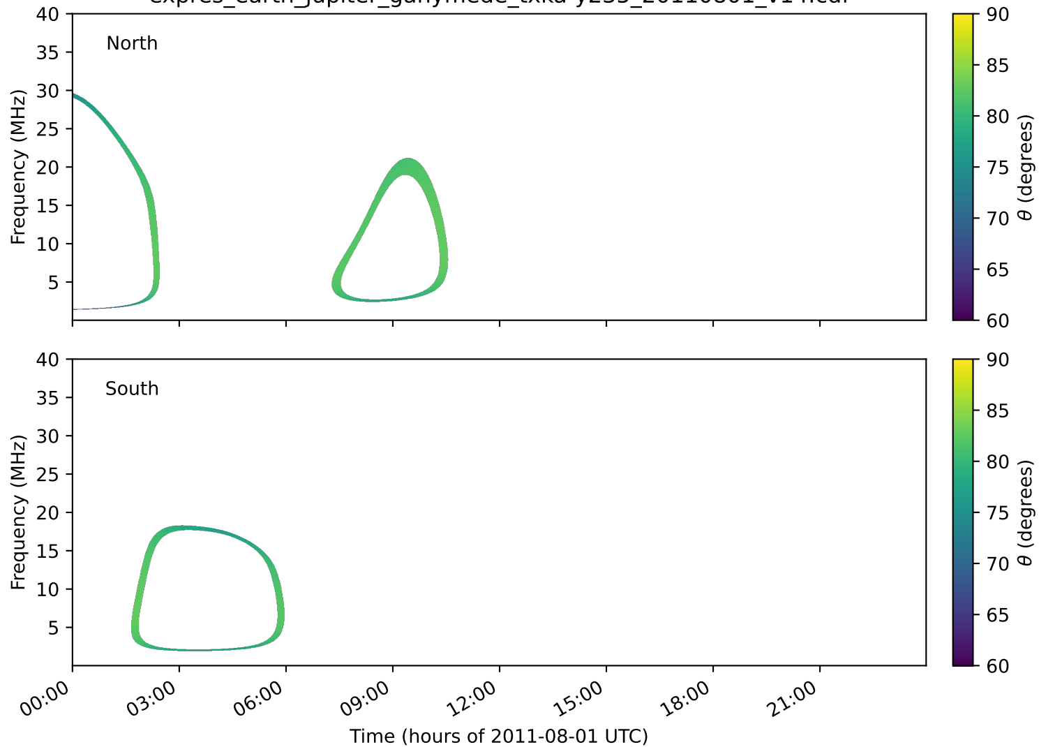
expres_earth_jupiter_ganymede_txka-y235_20110801_v14.cdf
