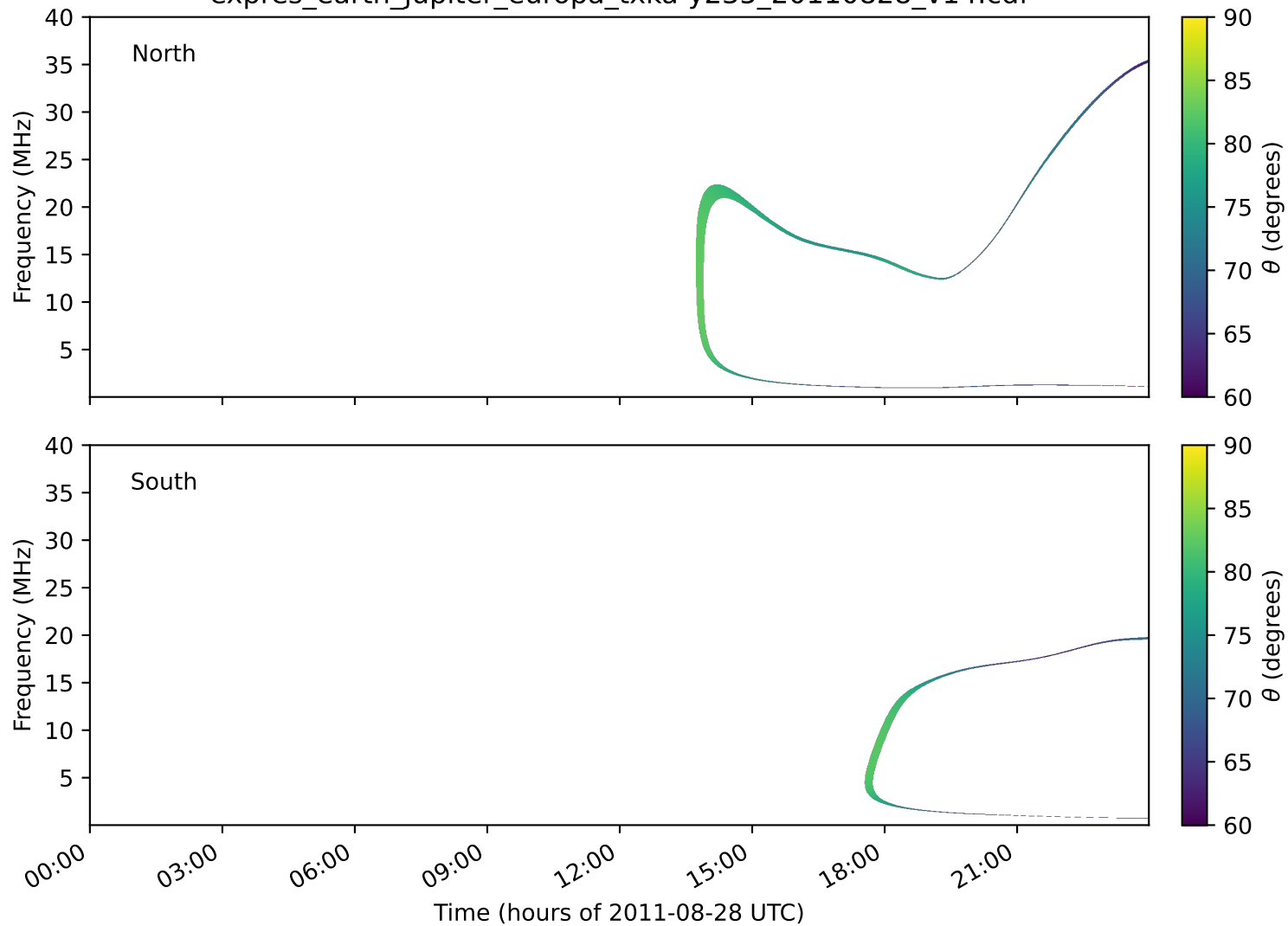
expres_earth_jupiter_europa_txka-y235_20110828_v14.cdf
