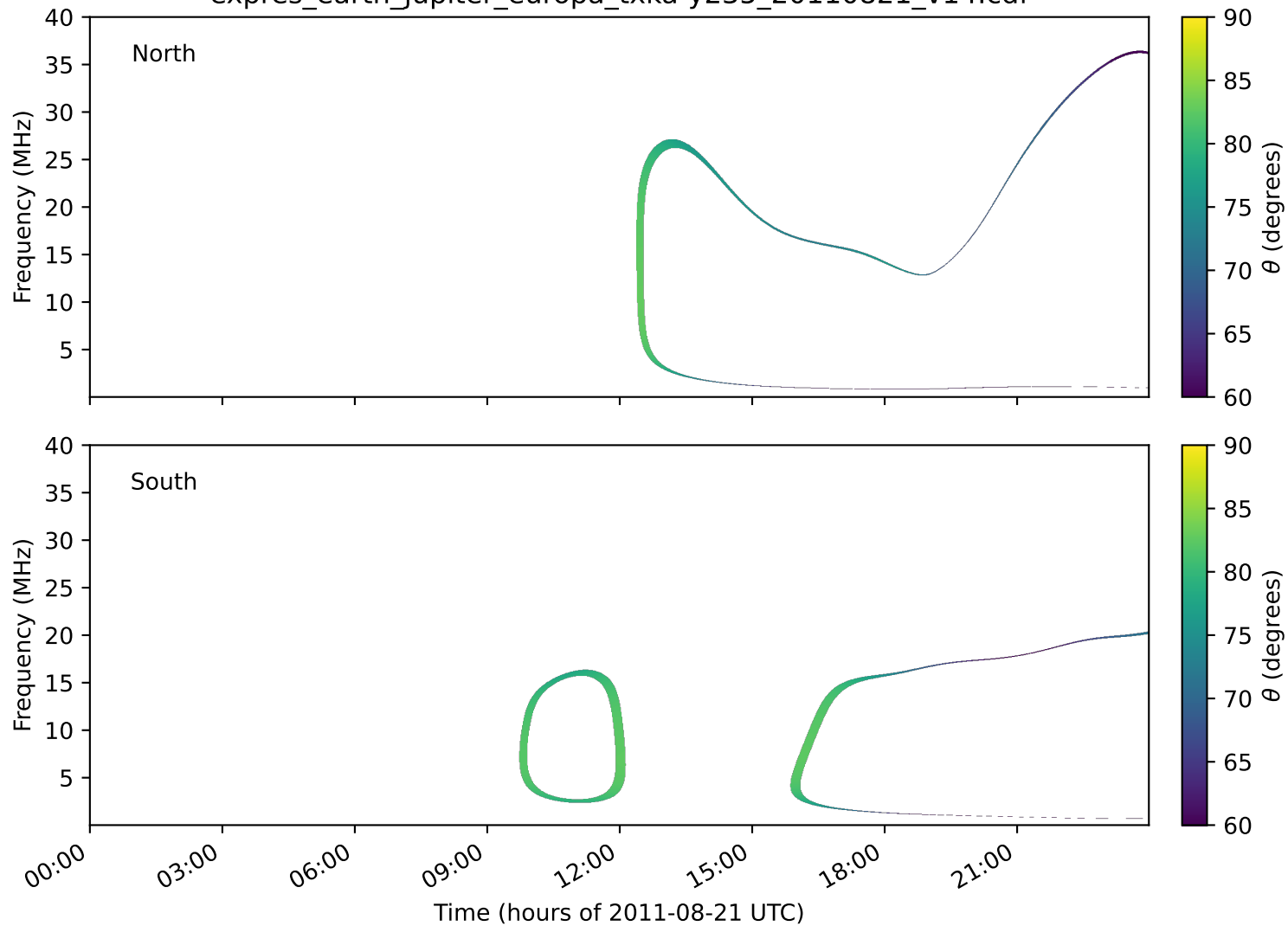
expres_earth_jupiter_europa_txka-y235_20110821_v14.cdf
