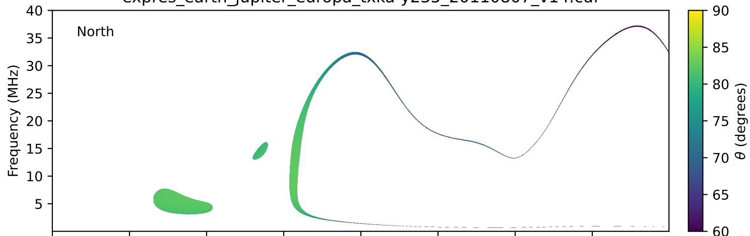
expres_earth_jupiter_europa_txka-y235_20110807_v14.cdf
