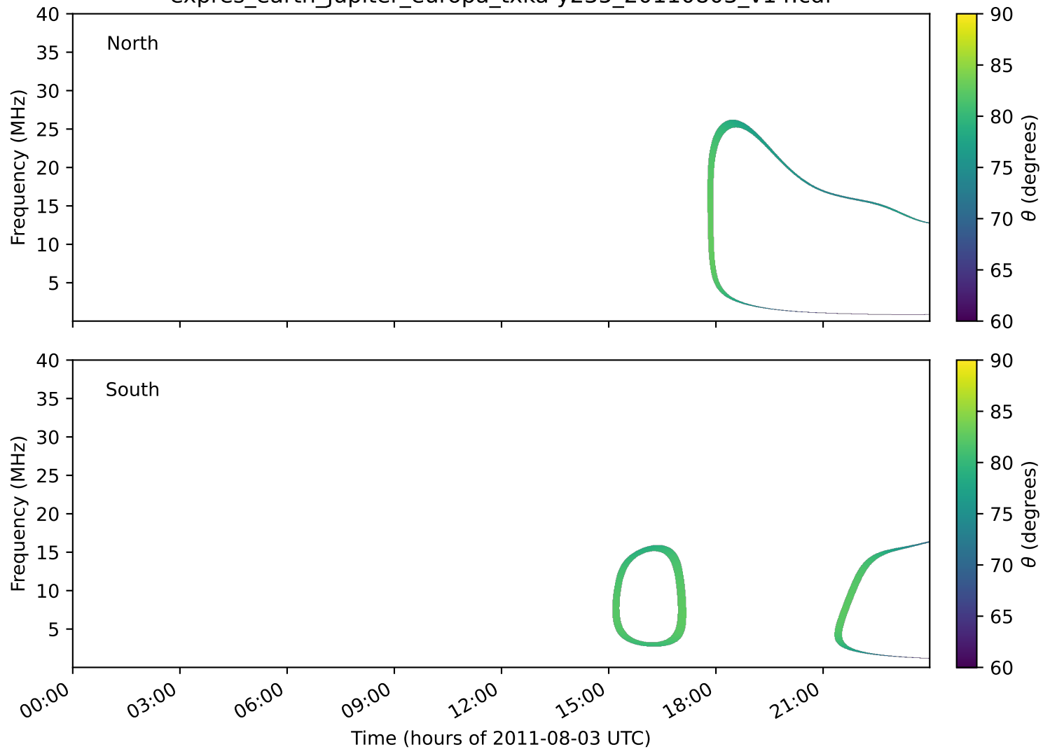
expres_earth_jupiter_europa_txka-y235_20110803_v14.cdf
