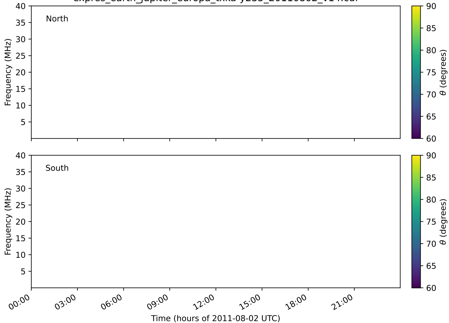
expres_earth_jupiter_europa_txka-y235_20110802_v14.cdf
