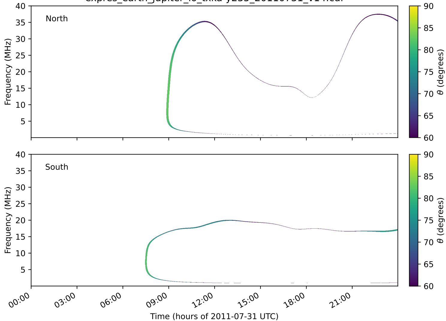
expres_earth_jupiter_io_txka-y235_20110731_v14.cdf
