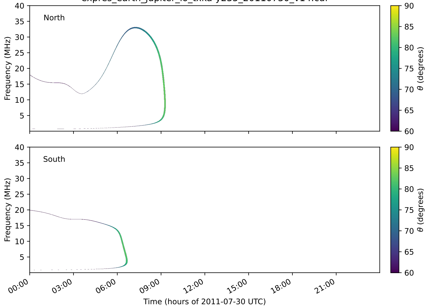
expres_earth_jupiter_io_txka-y235_20110730_v14.cdf
