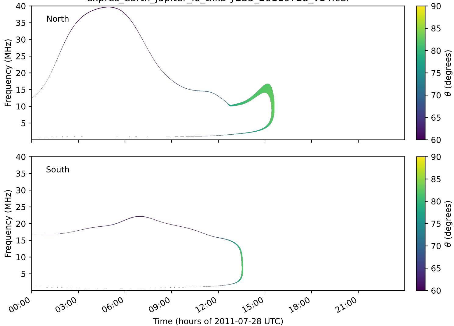
expres_earth_jupiter_io_txka-y235_20110728_v14.cdf
