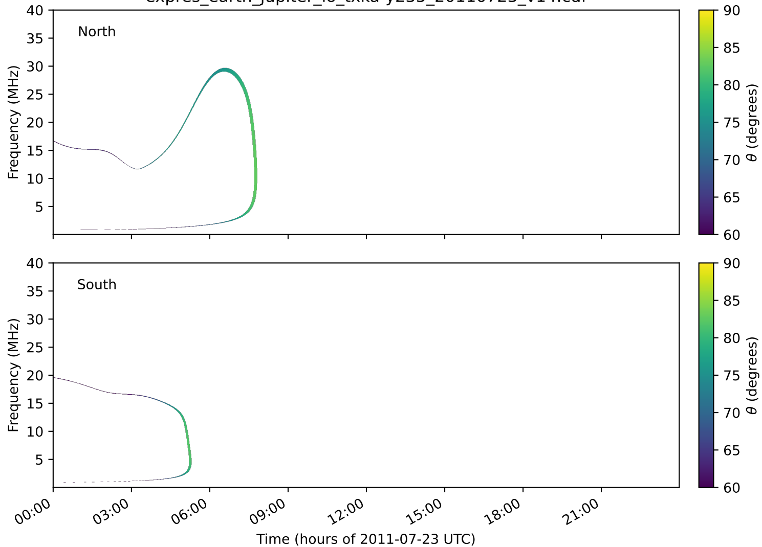
expres_earth_jupiter_io_txka-y235_20110723_v14.cdf
