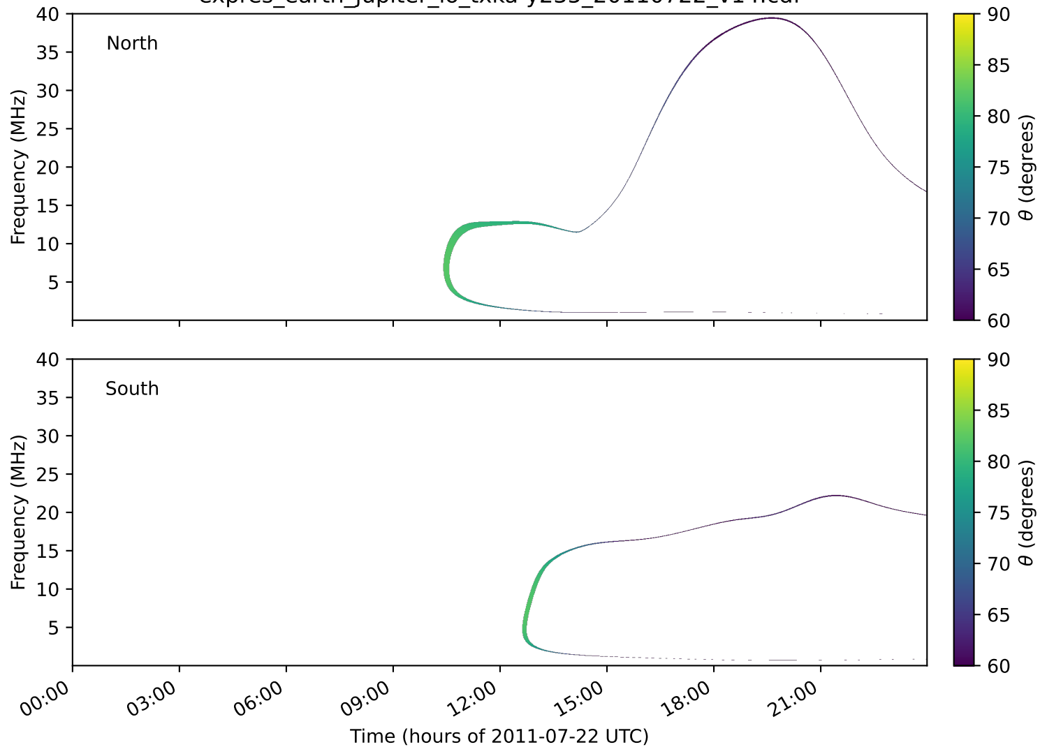
expres_earth_jupiter_io_txka-y235_20110722_v14.cdf
