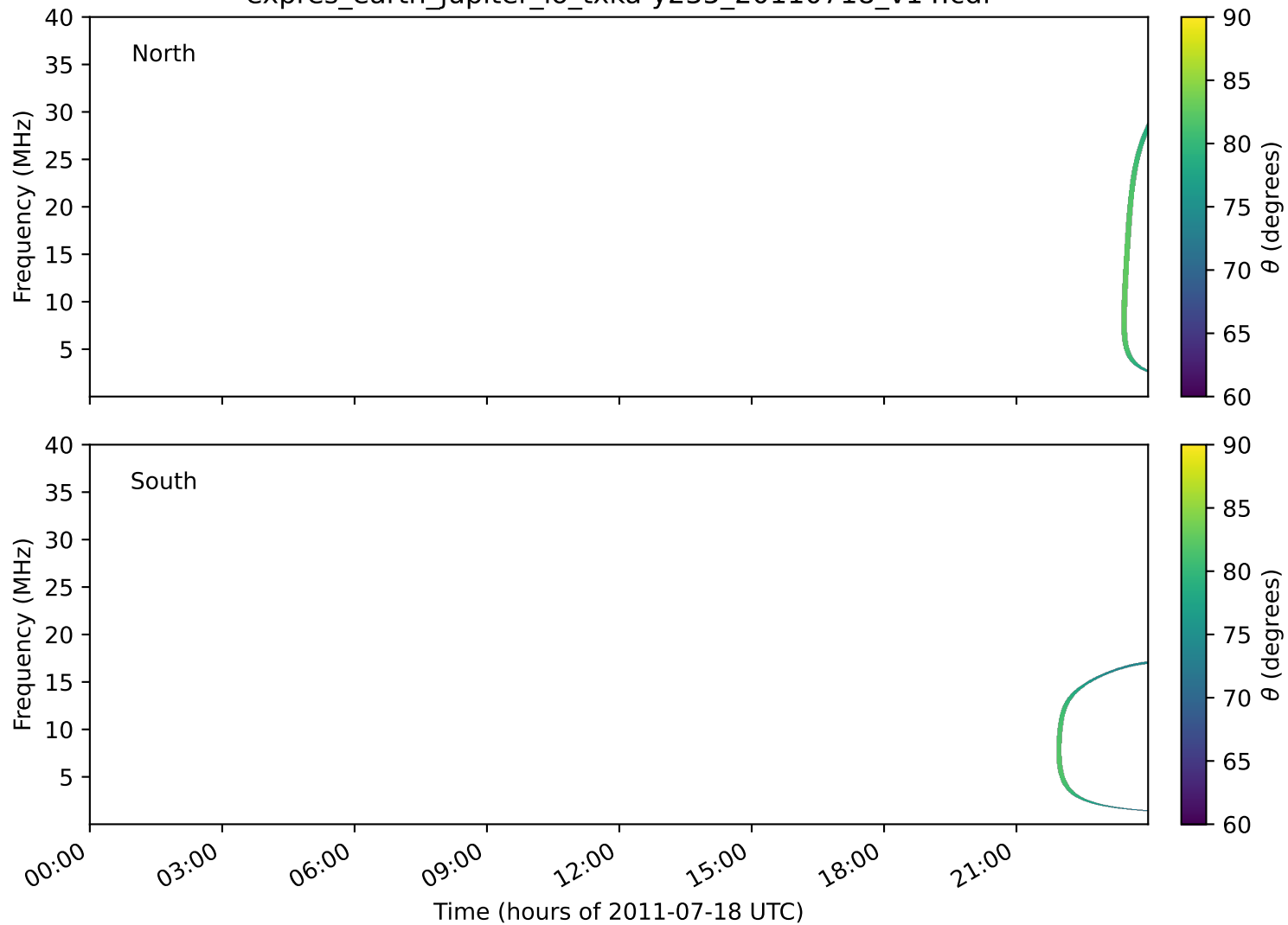
expres_earth_jupiter_io_txka-y235_20110718_v14.cdf
