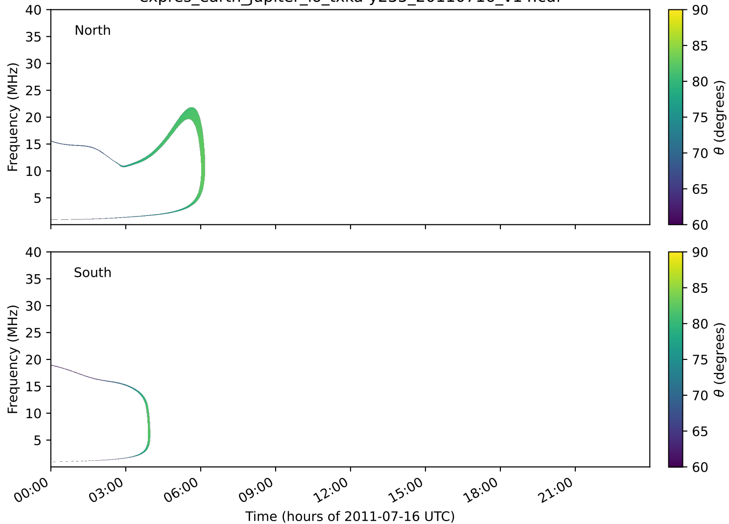
expres_earth_jupiter_io_txka-y235_20110716_v14.cdf
