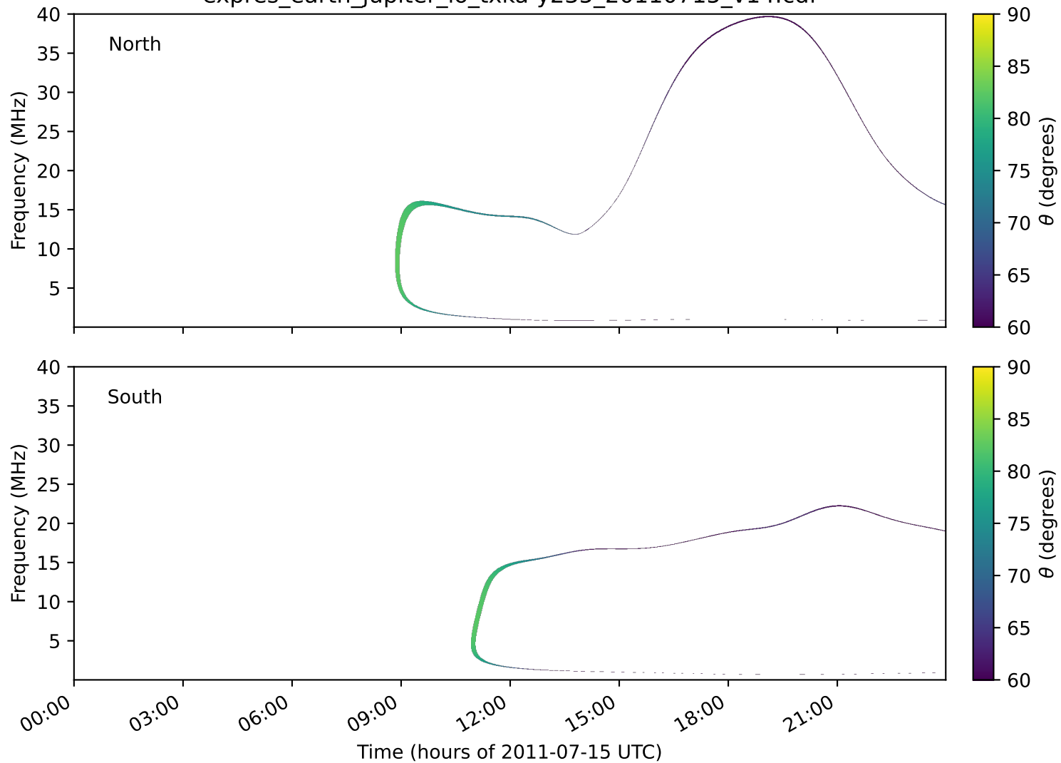
expres_earth_jupiter_io_txka-y235_20110715_v14.cdf
