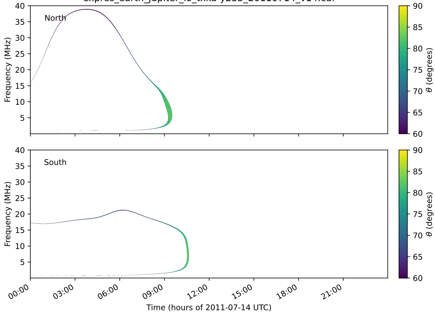
expres_earth_jupiter_io_txka-y235_20110714_v14.cdf
